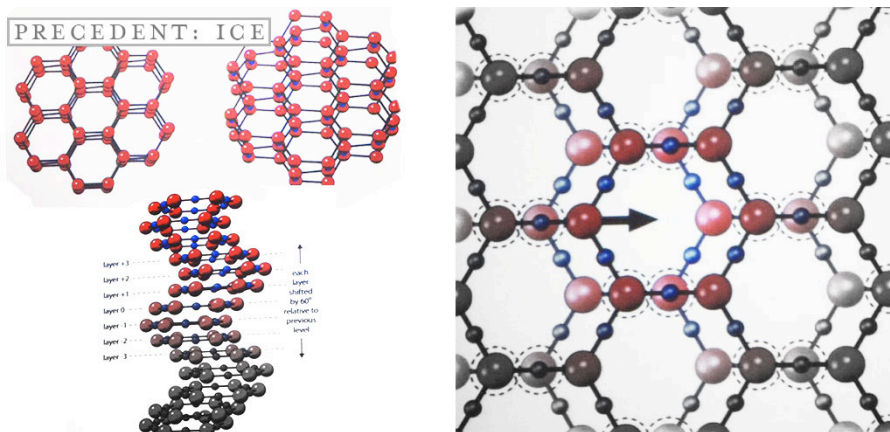
Figure 6. Hexagonal, or EZ structure of water (Pollack, 2013)
